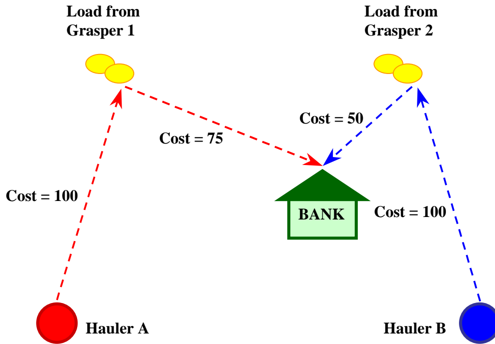
Figure 1: Two haulers bid on the loads from two graspers.
