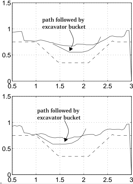
Fig. 7 Two digs. (a) and (b) show elevation profiles of the soil in testbed along the length of the trench that is to be created (marked by dashed lines). Forces at the bucket tip were measured at approximately 8 hz. \alpha_a = 25 degs, \alpha_b = 30 degs, d_{1a} = d_{1b} = 0.38 m, d_{2a} = d_{2b} = 0.26 m.
