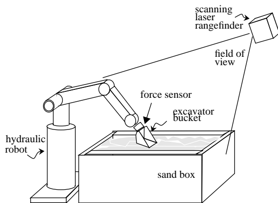
Fig. 5 Testbed
