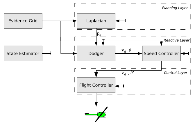
Fig. 6. Overall architecture of the algorithms. The higher the layer the lower the frequency of execution. A path p_g is produced in the planning layer and transmitted to the reactive layer. The reactive layer produces commands (v_d', \theta') that are then executed by the flight controller.
