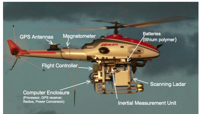
Fig. 12. The helicopter testbed, a Yamaha RMax, used for our experiments has a payload of 29kg besides fuel.
