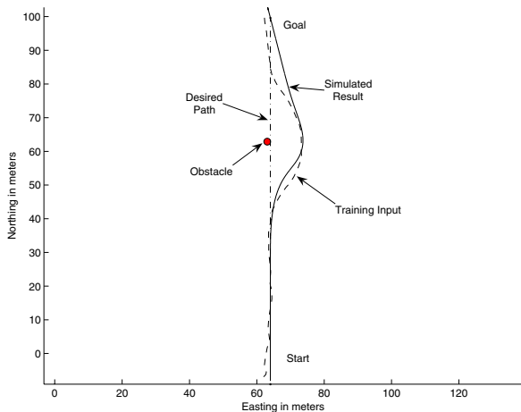
Fig. 10. This figure shows the desired path as a dot-dashed line, the path used for training as a dashed line and the simulated path as a solid line. The simulated path with the fine-tuned learned parameters still is a good match for our training path.
