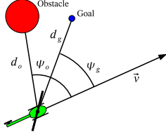
Fig. 7. A diagram illustrating the terms used in the control law. The coordinates used are expressed in a robot centric reference frame defined by the velocity and gravity vector.
