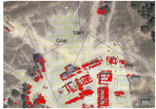
Fig. 5. A 2D (horizontal) slice of an evidence grid from the McKenna MOUT site at Ft. Benning, GA (USA). This model was created by flying part of the shown path. Red(Dark) represents occupancy and white is evidence of free space. An aerial image is overlaid on top of the evidence grid in order to facilitate the interpretation and show the accuracy of the constructed model. The grid spacing is 10m.
