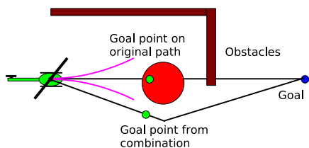
Fig. 11. Diagram illustrating the benefit of the combination of both algorithms. A new goal point is picked on the path from the planned trajectory. It avoids to potentially get stuck in a tight space that is occluded because the helicopter might have chosen to avoid the obstacle to the left.
