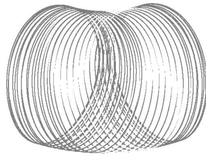
Fig. 2. Ladar scan pattern. The small circle is scanned at 22 Hz while it is swept across the field in 0.75s. This device provides range data at 64 kHz.
