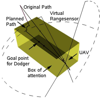
Fig. 9. A snapshot showing the box of attention and virtual field of view sensor. The box restricts the obstacles considered and is set between the dodger goal point and the current location of the UAV. The virtual range sensor is aligned with the current velocity vector.
