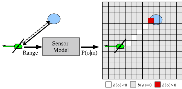
Fig. 4. A laser rangefinder returns a signal indicating a hit. The signal is mapped to a probability P(o|m) . This probability is used to update the relevant cells in the evidence grid.
