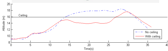
Fig. 14. Flying with and without ceiling when specified path is directly through a building. If a ceiling has been specified, the vehicle tries to stay below a specified altitude. On the run with ceiling, the system begins by flying around buildings, but then ignores altitude constraint and climbs to safely clear power lines. Key: Blue(dash-dot)→No ceiling. Red(solid)→With Ceiling.
