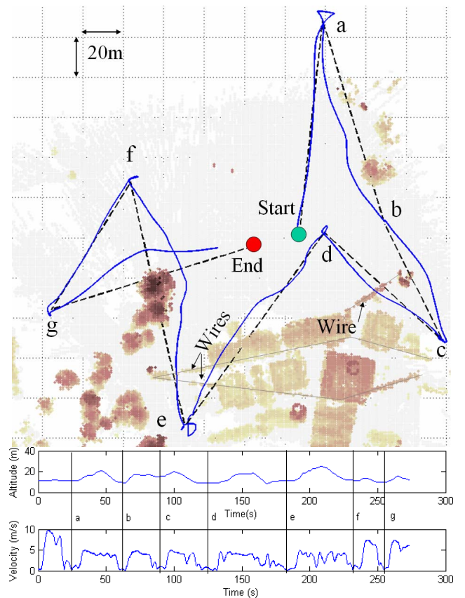
Fig. 13. A flight through the McKenna MOUT site at Ft. Benning at 4m/s. 8m/s was commanded at the first and 6m/s at the last two segments of the path.
