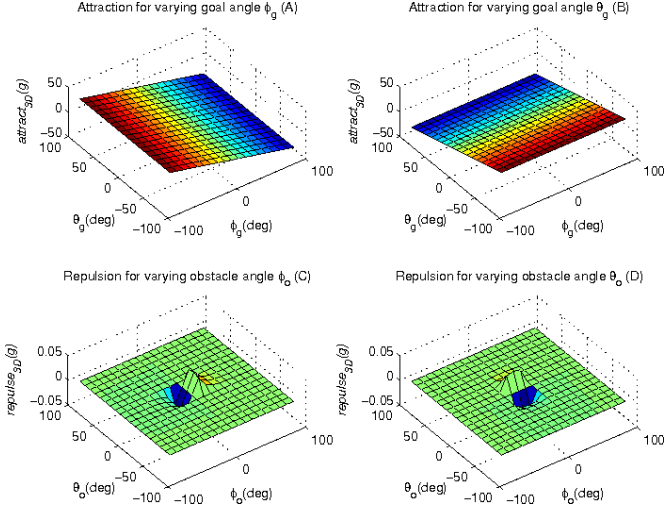
Fig. 8. The attraction and repulsion surface for our modified control law. Plot A and B show the independence of the goal attraction on each axis. Since a sigmoid shapes the repulsion for the repulsion function in plot C and D is not uniform.
